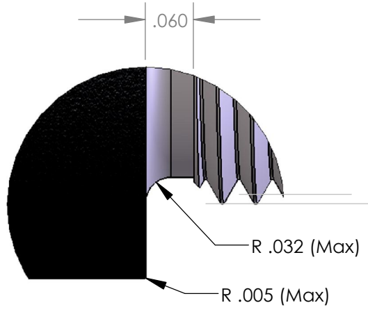
DETAIL E
